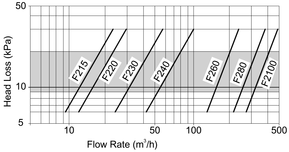
IMS 200 - Head Loss Graph
