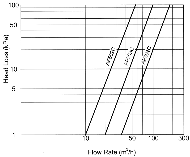
AF500C Head Loss Graph
