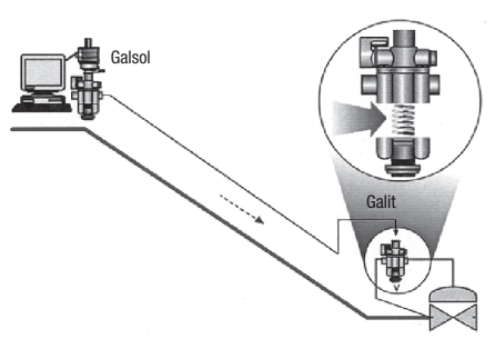
Solution For Topographic Height Difference
