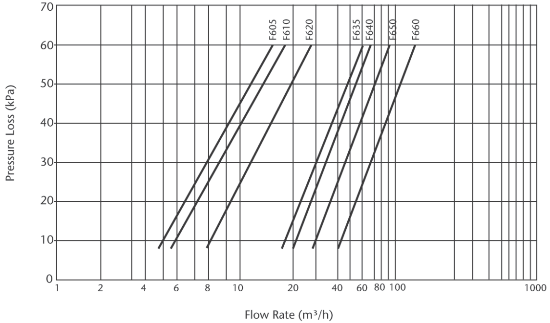
600 Series Head Loss Graph (per tank)
